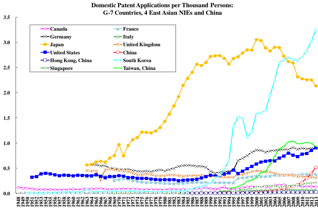
Chart 5: Domestic Patent Applications Filed Annually per Thousand Persons: G-7 Countries, 4 EANIEs and China
